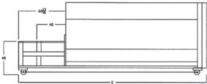
• 34 CUBIC YARD IS 22'-11" -- 30 CUBIC YARD IS 21'-5"
